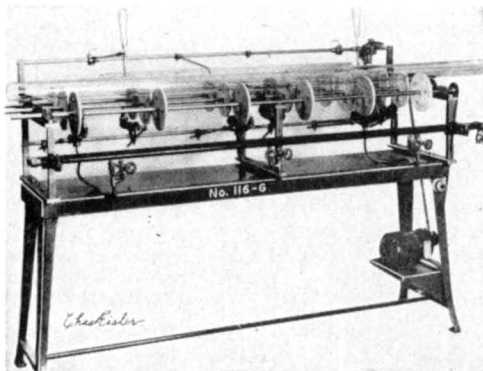
The Eisler glass tube-cracking-off machine. (Patent No. 2,410,931.)
